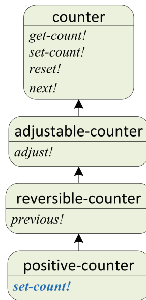
Figure 10.3. Counter class hierarchy.
