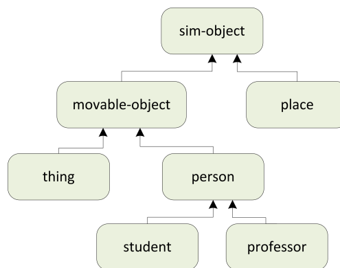
Figure 10.2. Inheritance Hierarchy.
